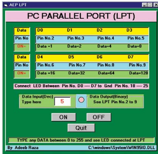
Fig. 4: Screen that appears when program is run
