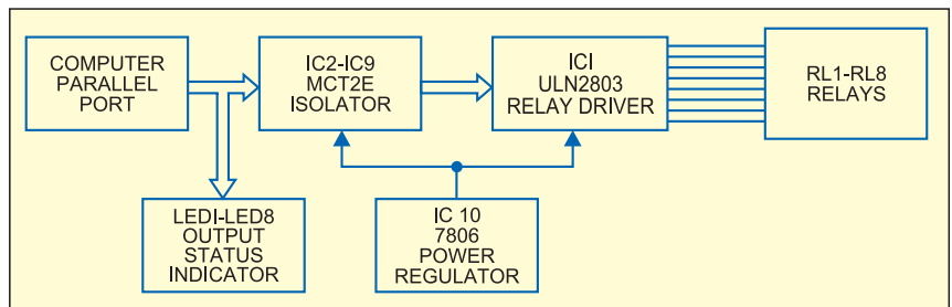
Fig. 1: Block diagram of device control through PC's parallel port using Visual Basic
